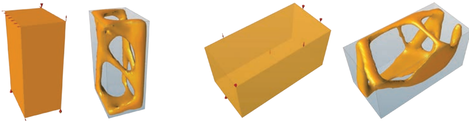
Morphology exploration based on stress optimization in Inspire. Vida Chang, M.Arch, Pratt Institute 2012.
