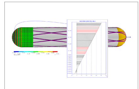
Composite pressure vessel analysis
