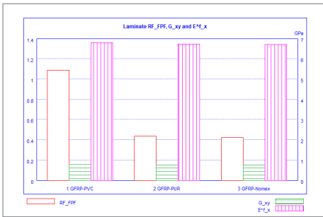
Comparison of laminate properties
