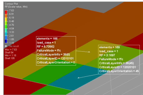
In-depth failure information for Altair HyperView™
